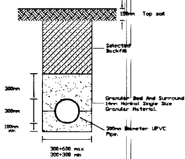
SURFACE WATER DRAIN BEDDING DETAIL A Not To Scale
