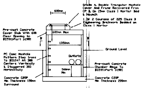
DETAILS OF CATCH PIT CP D SECTION A - A Not To Scale
