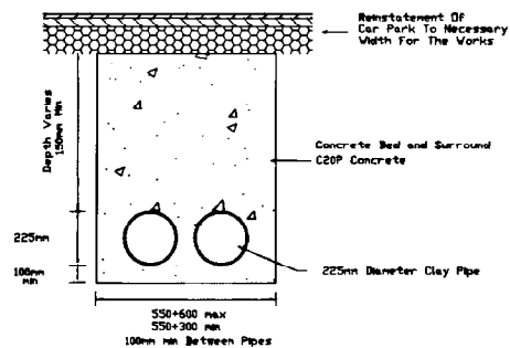
SURFACE WATER DRAIN BEDDING DETAIL B Not To Scale
