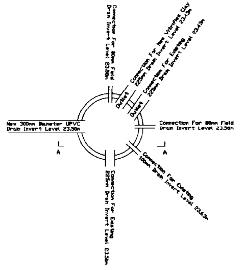
DETAILS OF CATCH PIT CP D PLAN B - B Not To Scale
