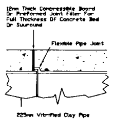
EXPANSION JOINT DETAIL FOR CONCRETE SURROUND
